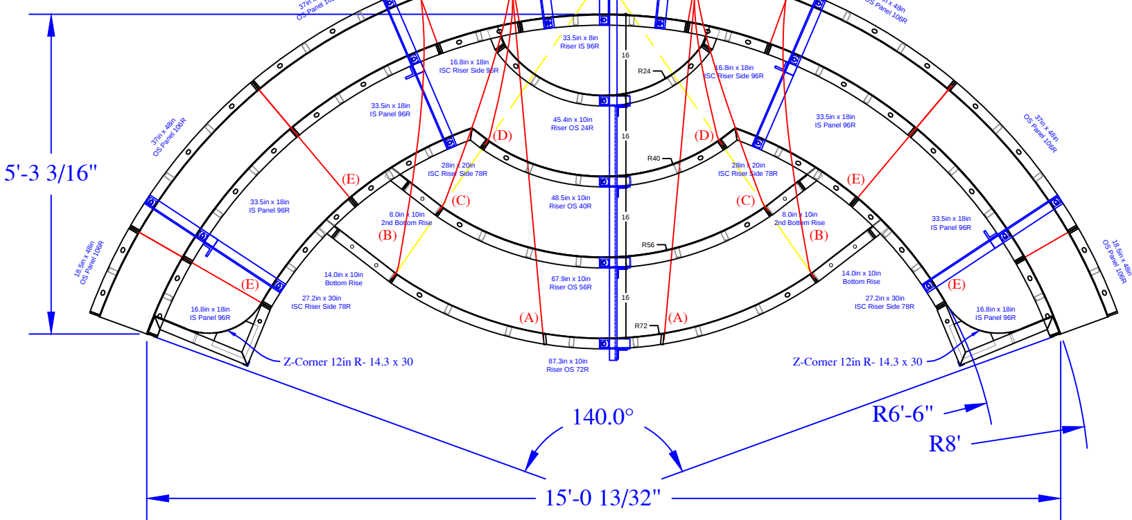
(E) Qty (8) - 27 7/8" Wall Tie - Middle Rise 1/4" BB
