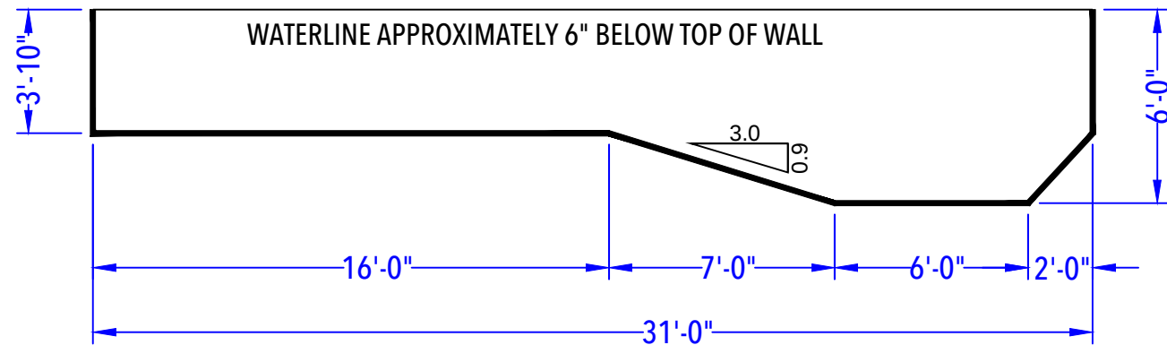
DEPTH DETAIL
