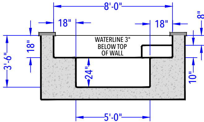
8' x 8' SQUARE RAISED SPILLOVER SPA PLAN & ELEVATION VIEW (After Concrete & Plaster)
