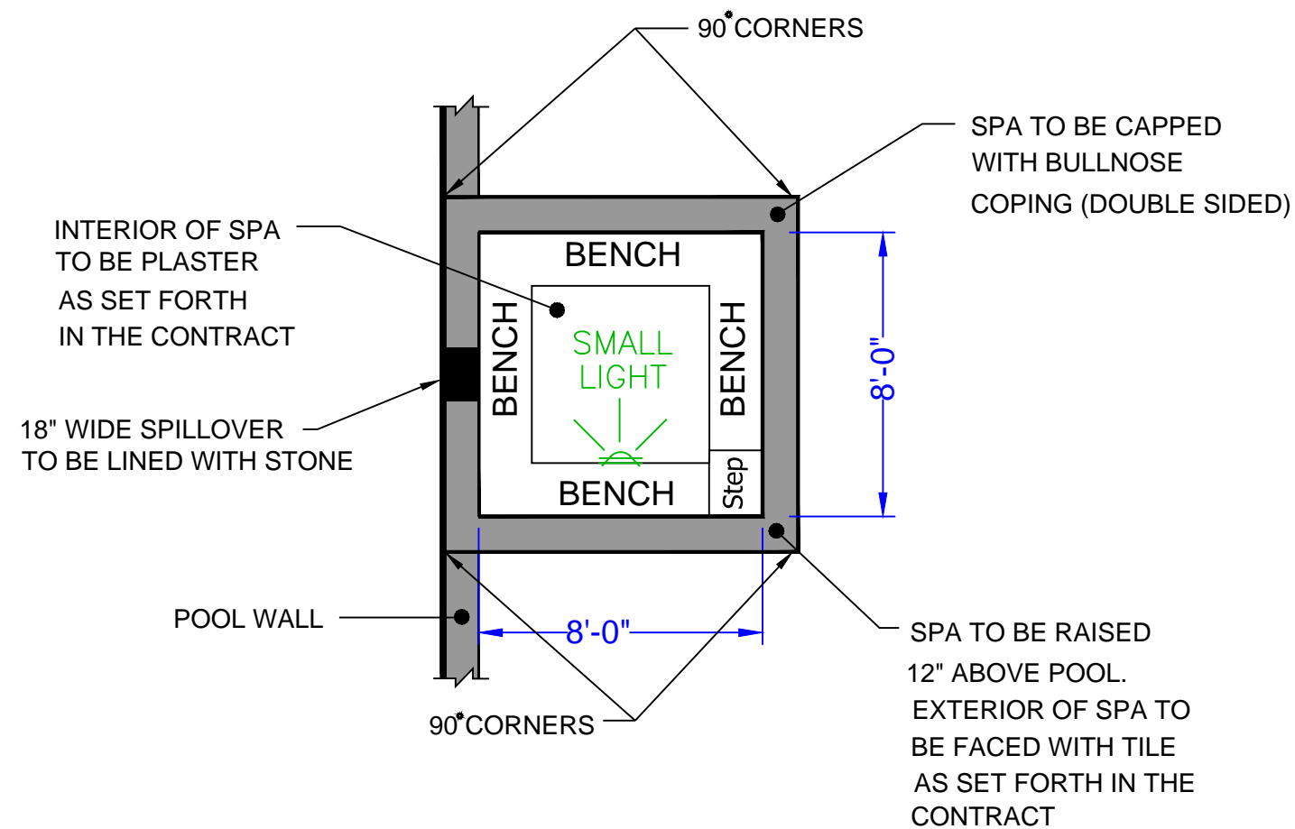
8' x 8' RAISED SPILLOVER SPA DETAIL (After Concrete & Plaster) N.T.S
