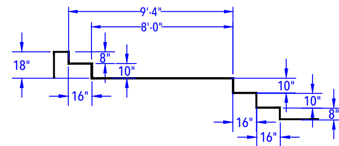
SUN DECK / STEP DETAIL (After Bottom & Liner) N.T.S.
