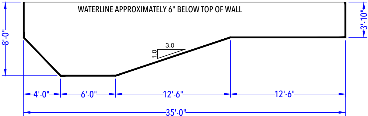
DEPTH DETAIL
