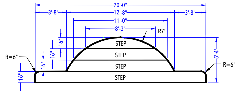
ENTRY STEP DETAIL (After Concrete & Liner) N.T.S.
