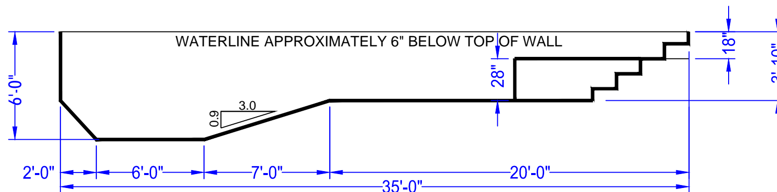
DEPTH DETAIL
