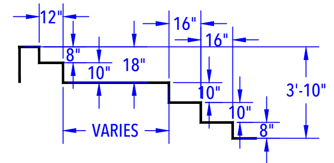
SUNDECK / ENTRY STEP DETAIL (After Bottom & Liner) N.T.S.
