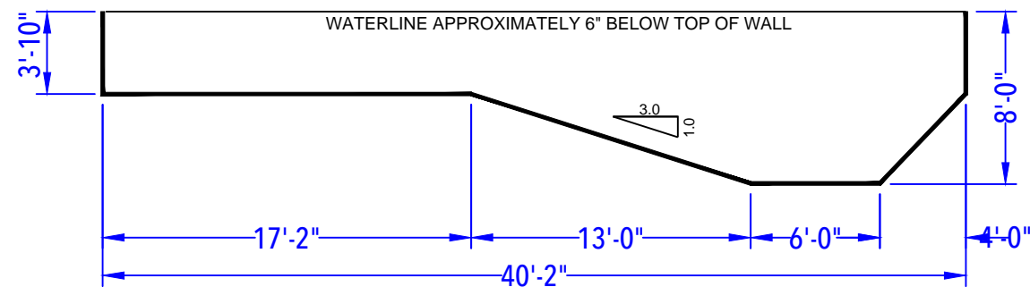
DEPTH DETAIL
