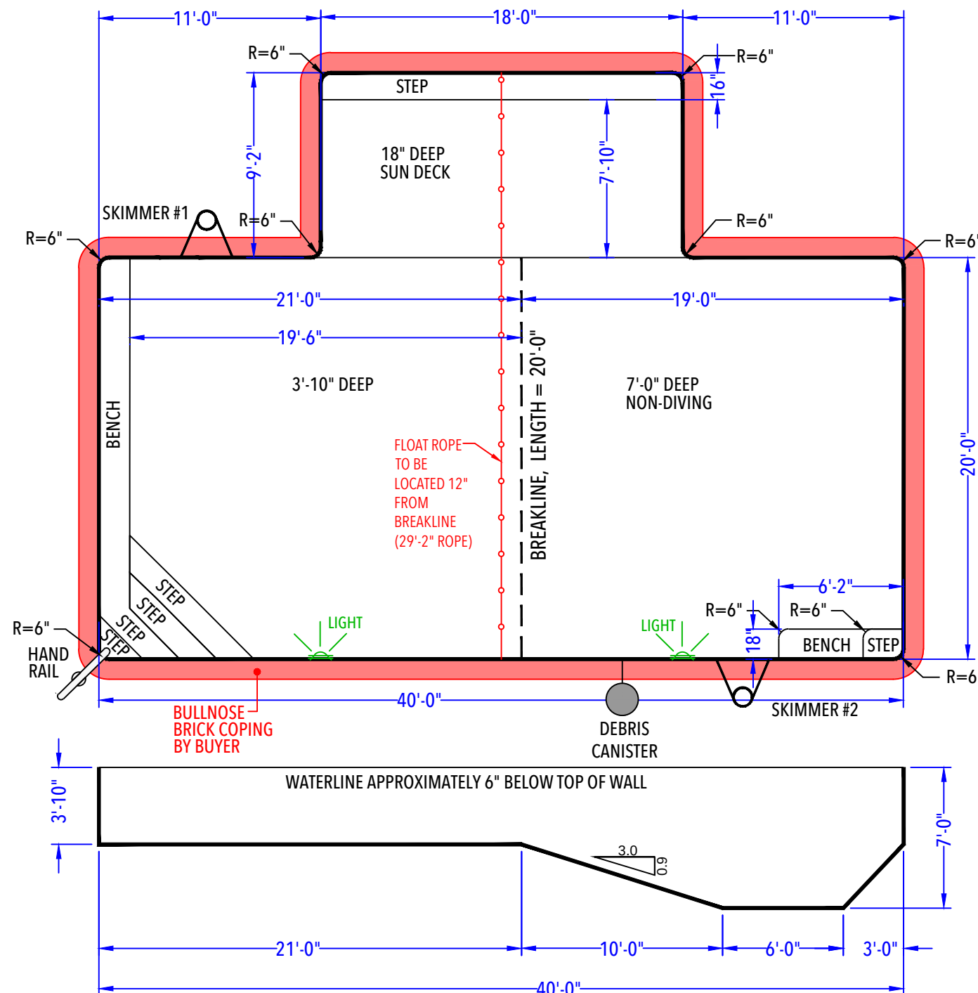
DEPTH DETAIL
