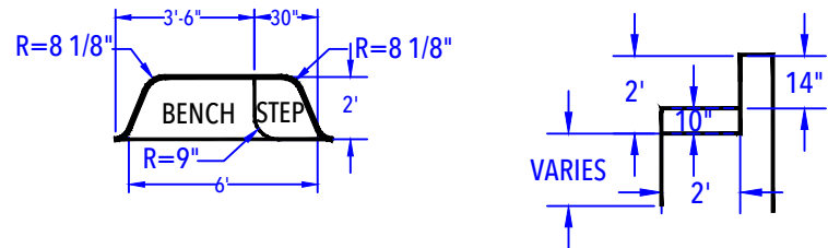
DEEP END BENCH & STEP OUT DETAIL (After Concrete & Liner) N.T.S.
