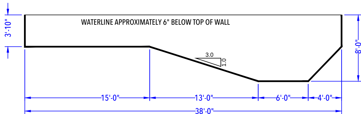
DEPTH DETAIL
