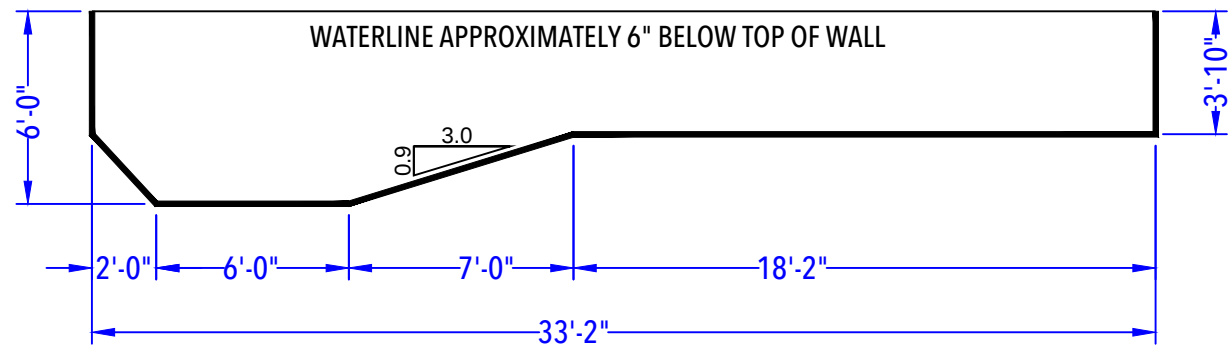
DEPTH DETAIL
