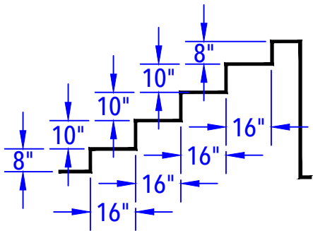
ENTRY STEP DETAIL (After Concrete & Liner) N.T.S.
