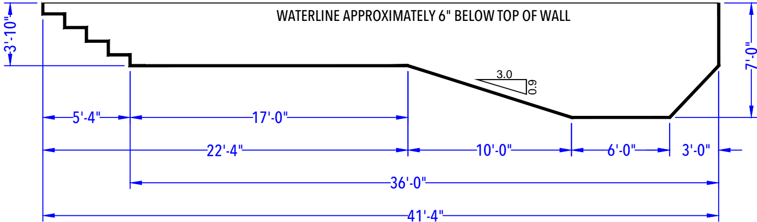
DEPTH DETAIL
