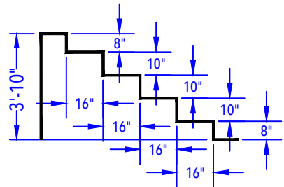
ENTRY STEP DETAIL (After Concrete & Liner) N.T.S.
