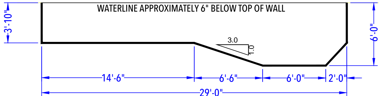
DEPTH DETAIL
