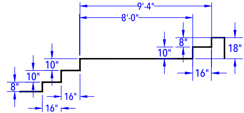
SUN DECK & ENTRY STEP DETAIL (After Concrete & Liner)
