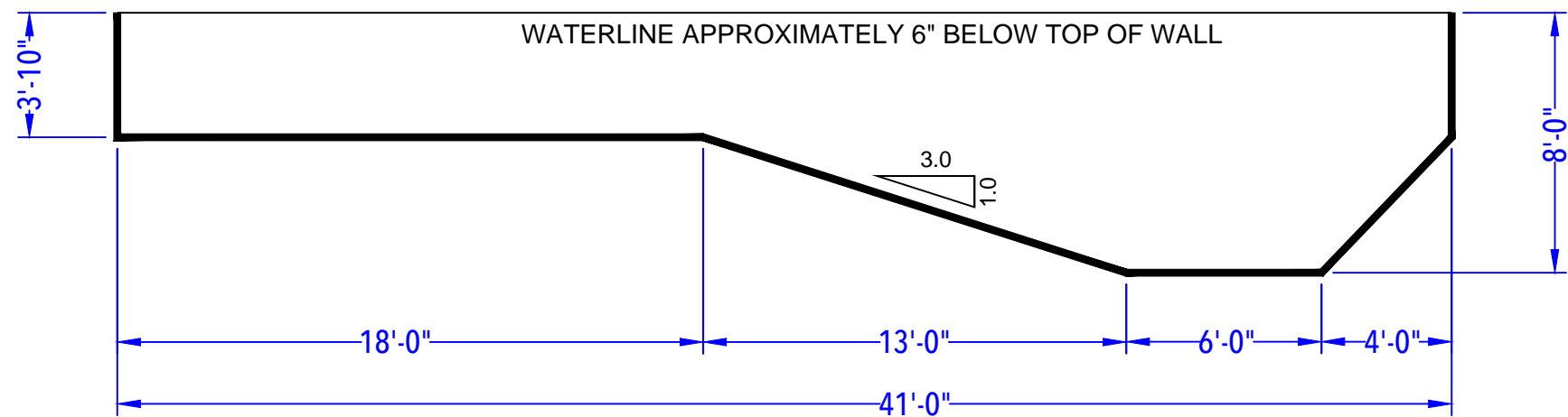
DEPTH DETAIL
