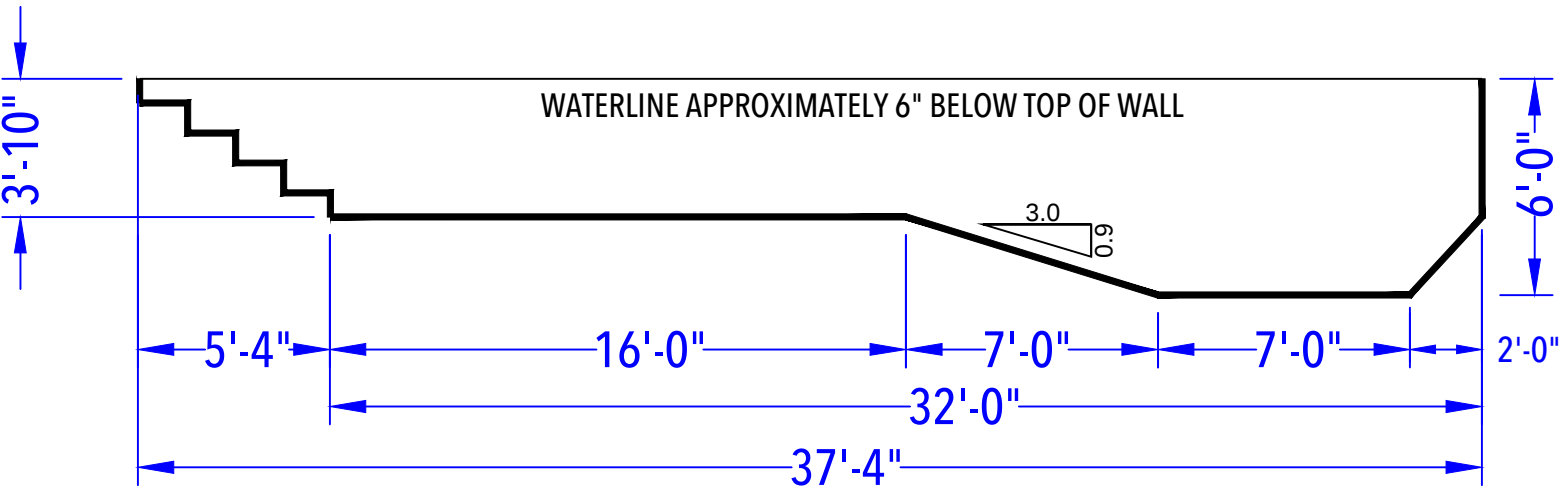
DEPTH DETAIL
