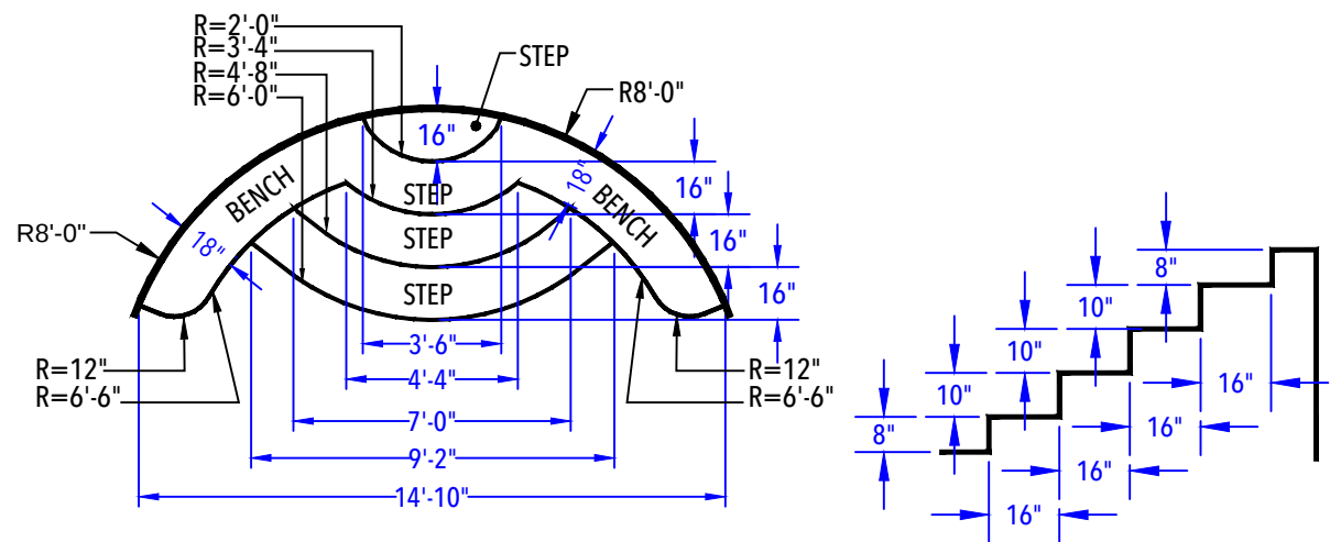
ENTRY STEP DETAIL (After Concrete & Liner) N.T.S.
