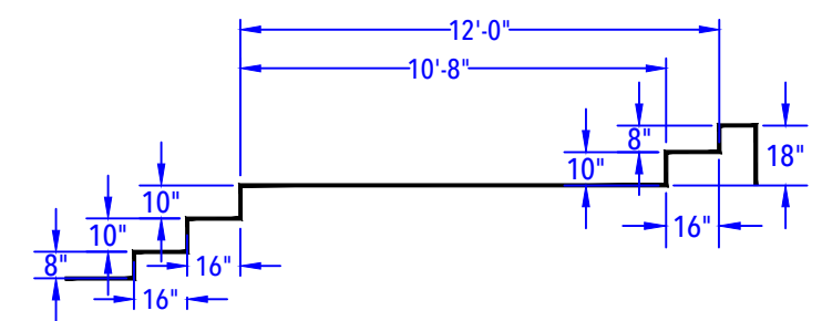
SUN DECK + STEP COMBO DETAIL (After Concrete & Liner) N.T.S.
