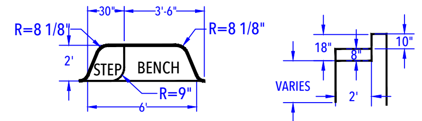
DEEP END BENCH + STEP OUT DETIAL (After Concrete & Liner) N.T.S.
