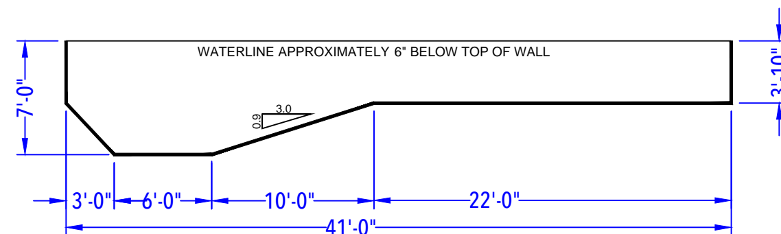
DEPTH DETAIL
