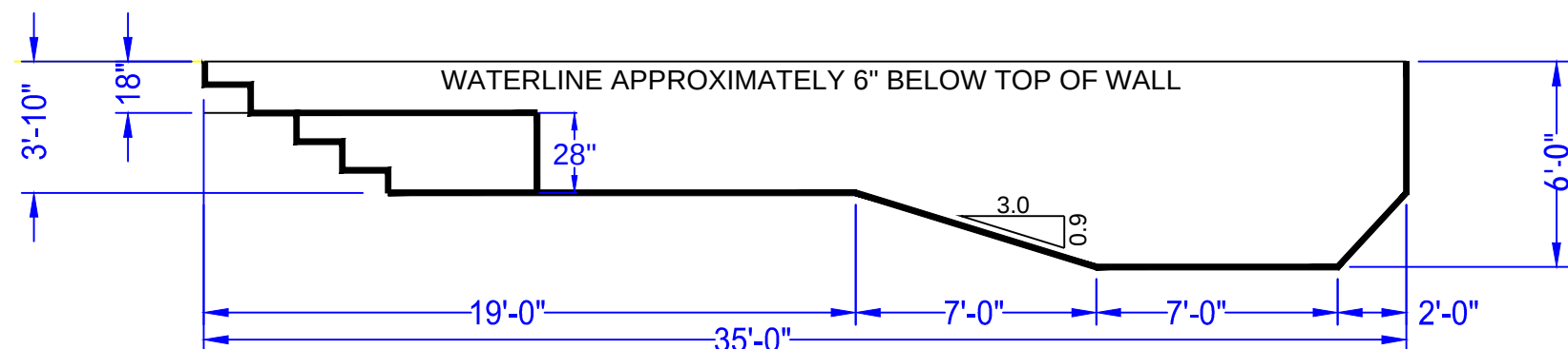
DEPTH DETAIL
