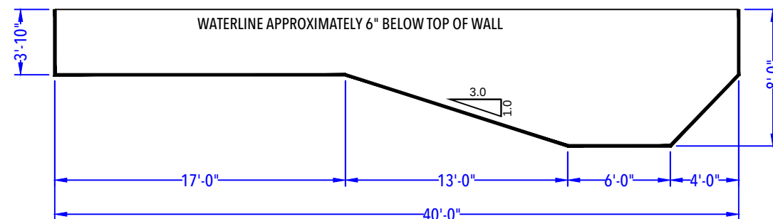
DEPTH DETAIL
