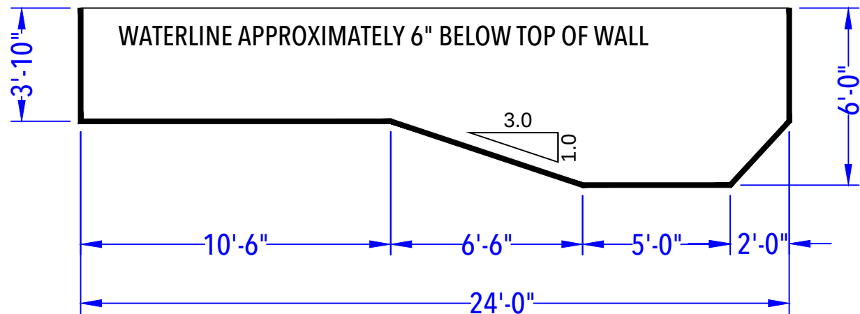
DEPTH DETAIL
