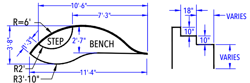
DEEP END BENCH & STEP OUT DETAIL
