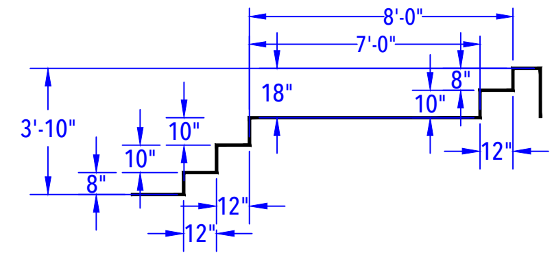
SUN DECK & ENTRY STEP DETAIL
