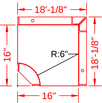
CORNER DETAIL
