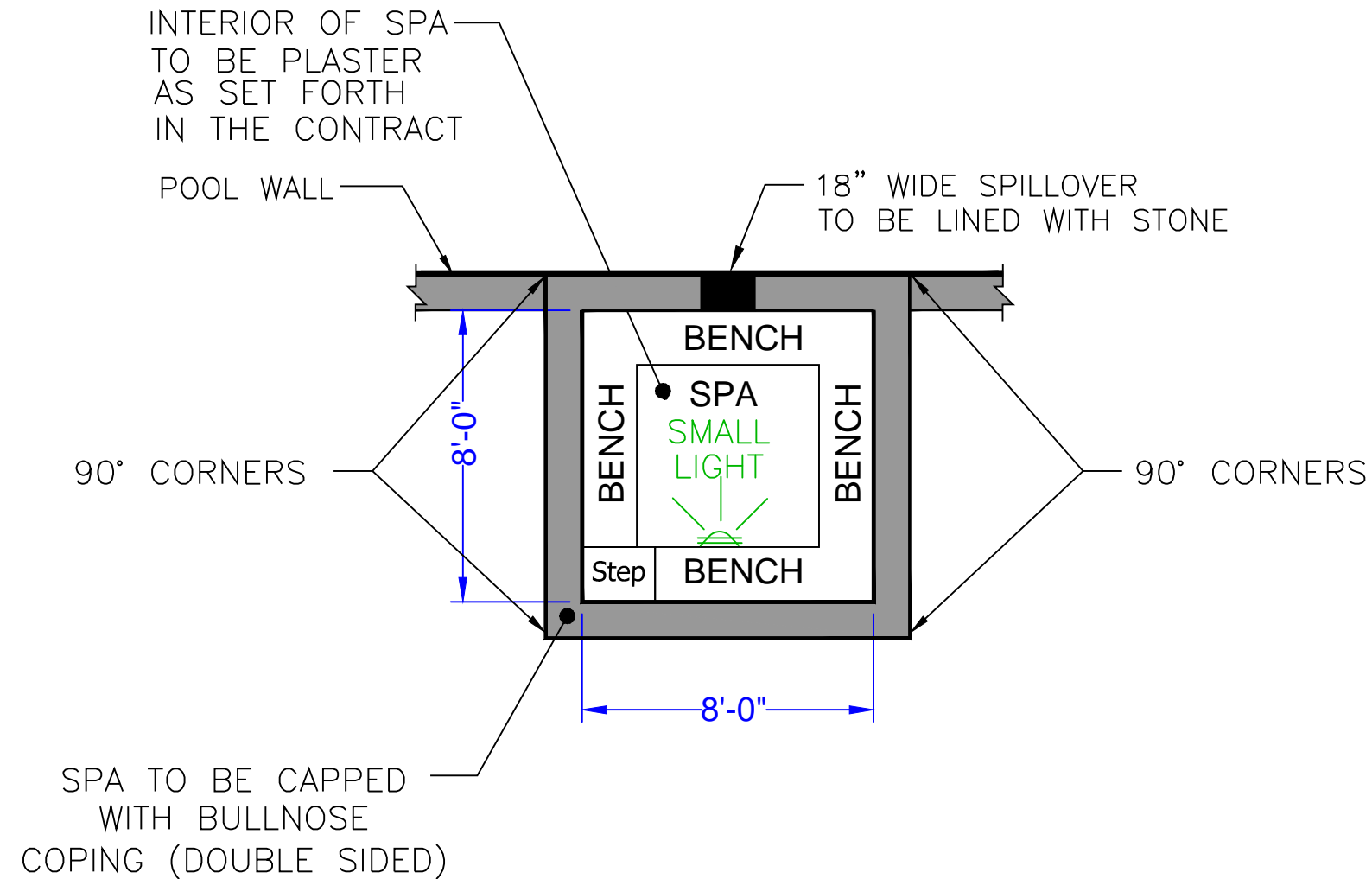
SPA DETAIL (After Concrete & Plaster) N.T.S
