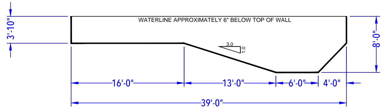
DEPTH DETAIL
