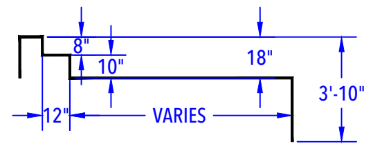
SUN DECK DETAIL (After Concrete & Liner) N.T.S.
