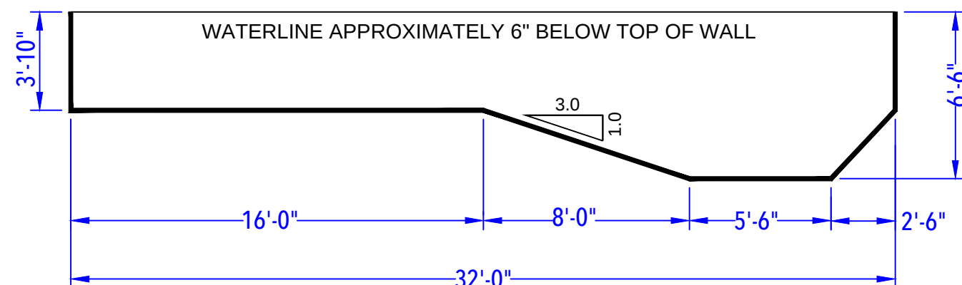
DEPTH DETAIL
