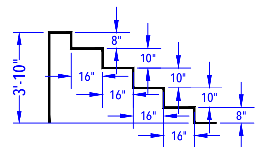
ENTRY STEP DETAIL (After Concrete & Liner) N.T.S.
