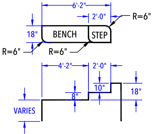
DEEP END BENCH & STEP OUT DETAIL (After Concrete & Liner) N.T.S.
