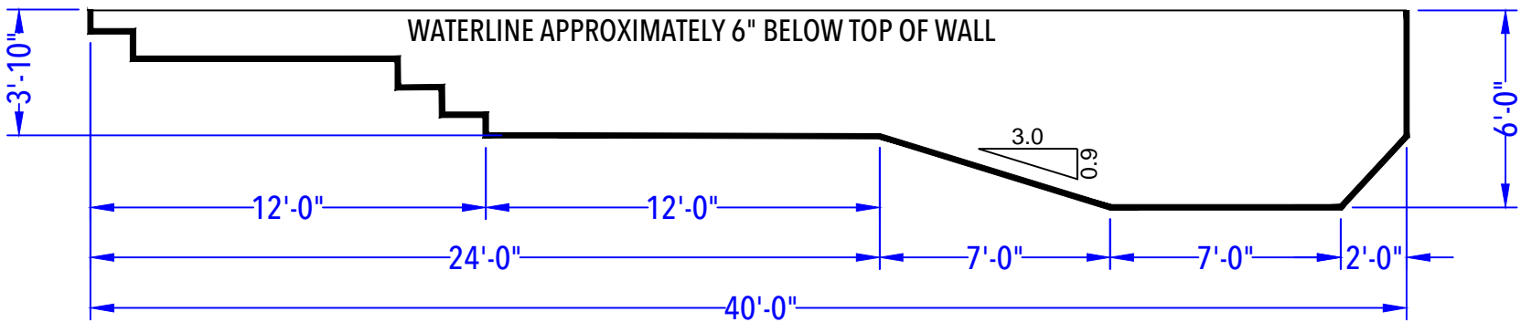
DEPTH DETAIL
