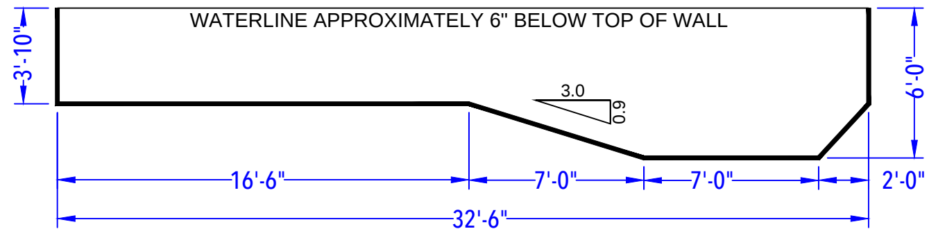
DEPTH DETAIL
