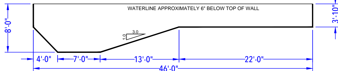
DEPTH DETAIL
