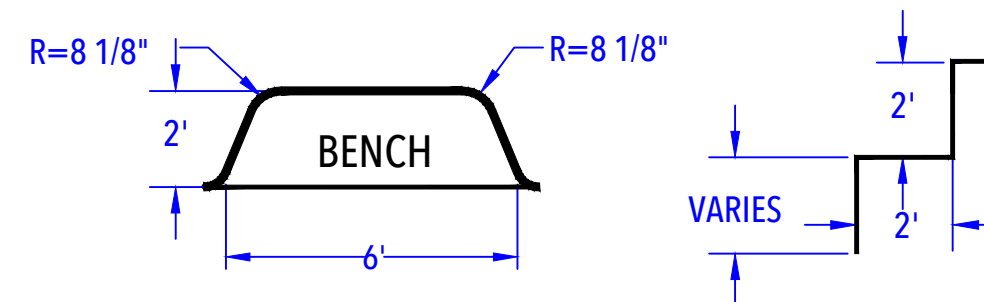
DEEP END BENCH DETAIL (After Bottom & Liner) N.T.S.
