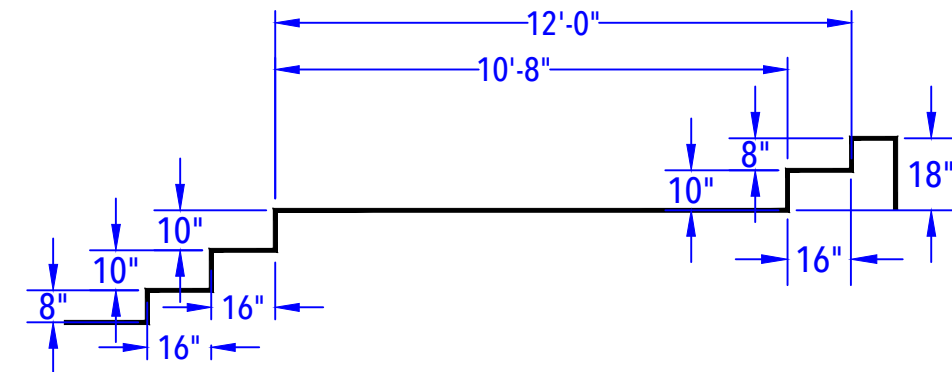
SUNDECK / STEP DETAIL (After Bottom & Liner) N.T.S.
