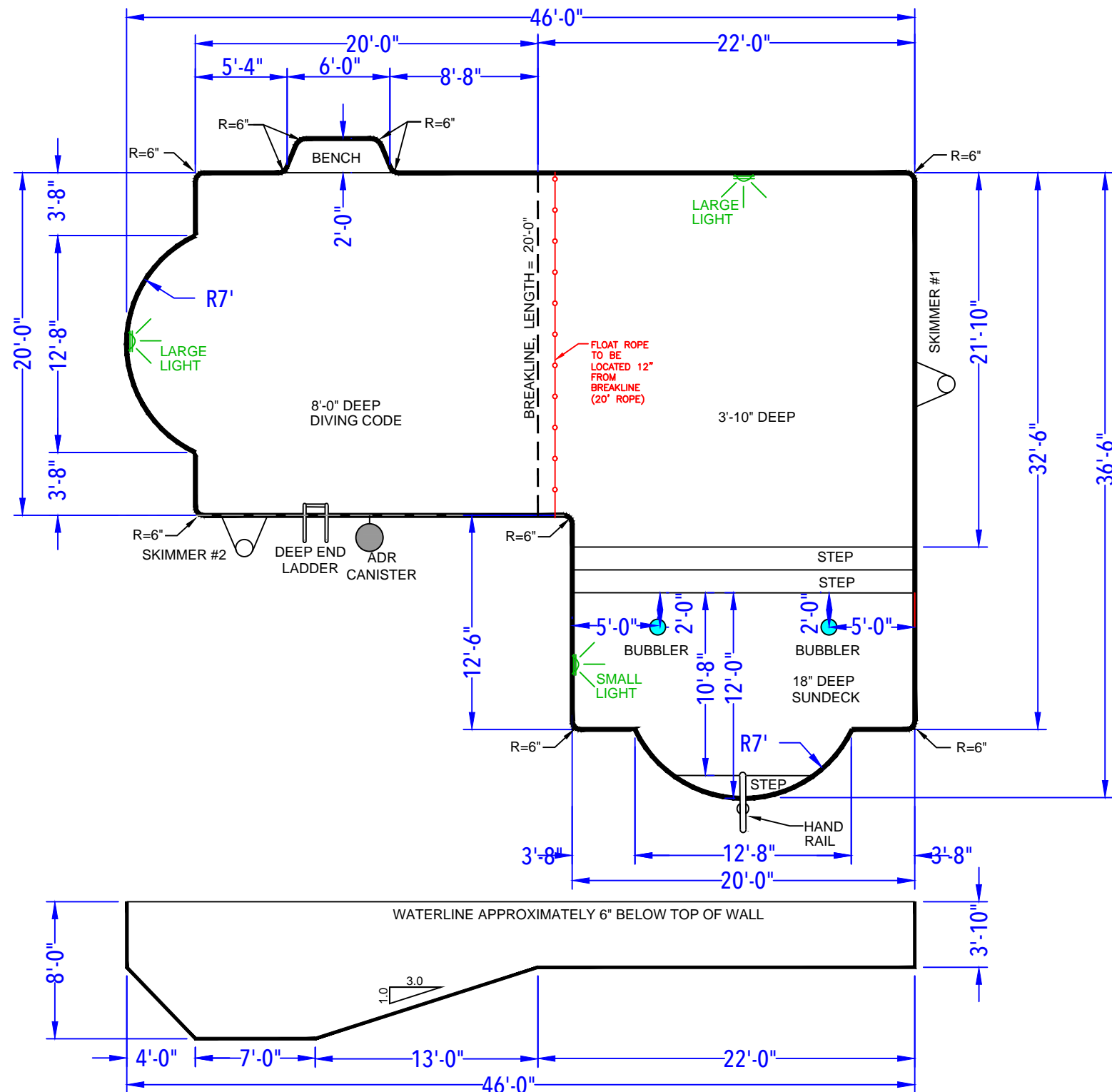
DEPTH DETAIL
