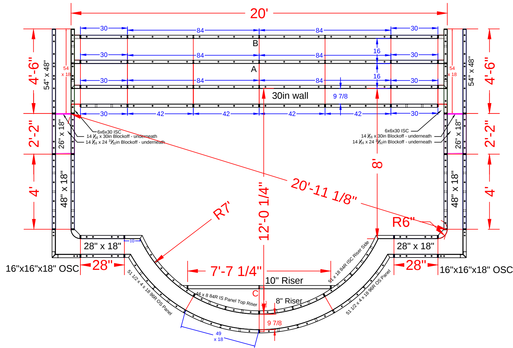
20' WIDE ROMAN END SUNDECK DETAIL SCALE: 1' = 1 / 3 "
