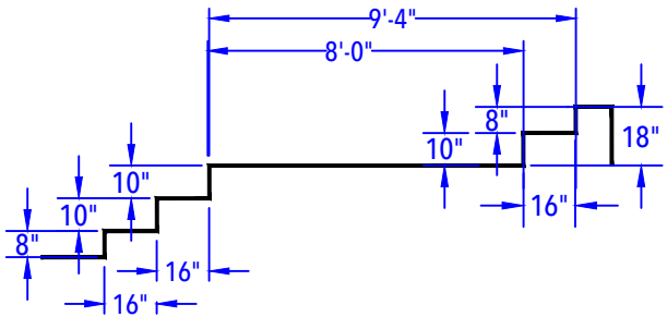
SUN DECK & STEP DETAIL (After Concrete & Liner) N.T.S.
