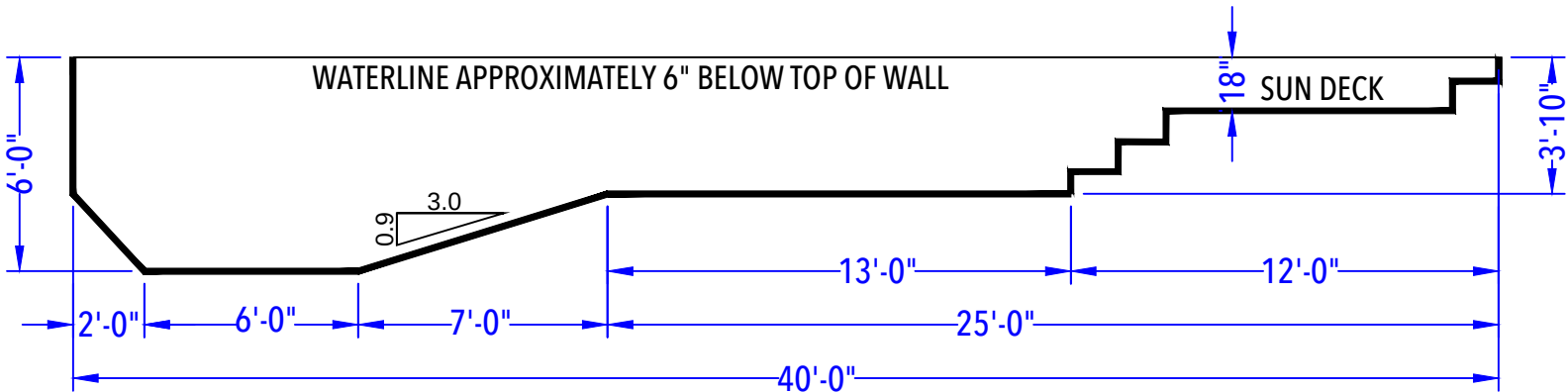
DEPTH DETAIL
