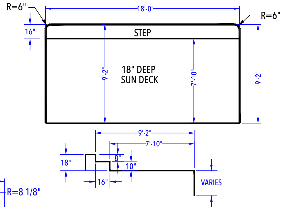
SIDE SUN DECK DETAIL (After Concrete & Liner) N.T.S.
