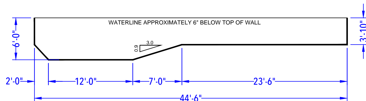
DEPTH DETAIL
