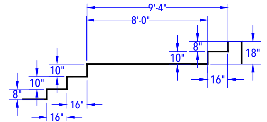
SUNDECK / STEP DETAIL (After Bottom & Liner) N.T.S.
