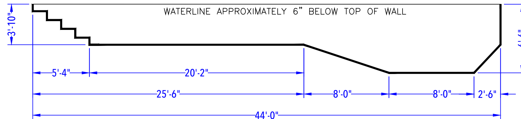
DEPTH DETAIL
