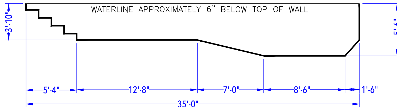
DEPTH DETAIL
