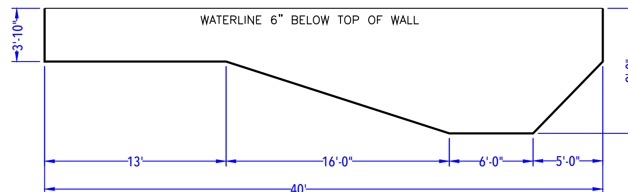
DEPTH DETAIL
