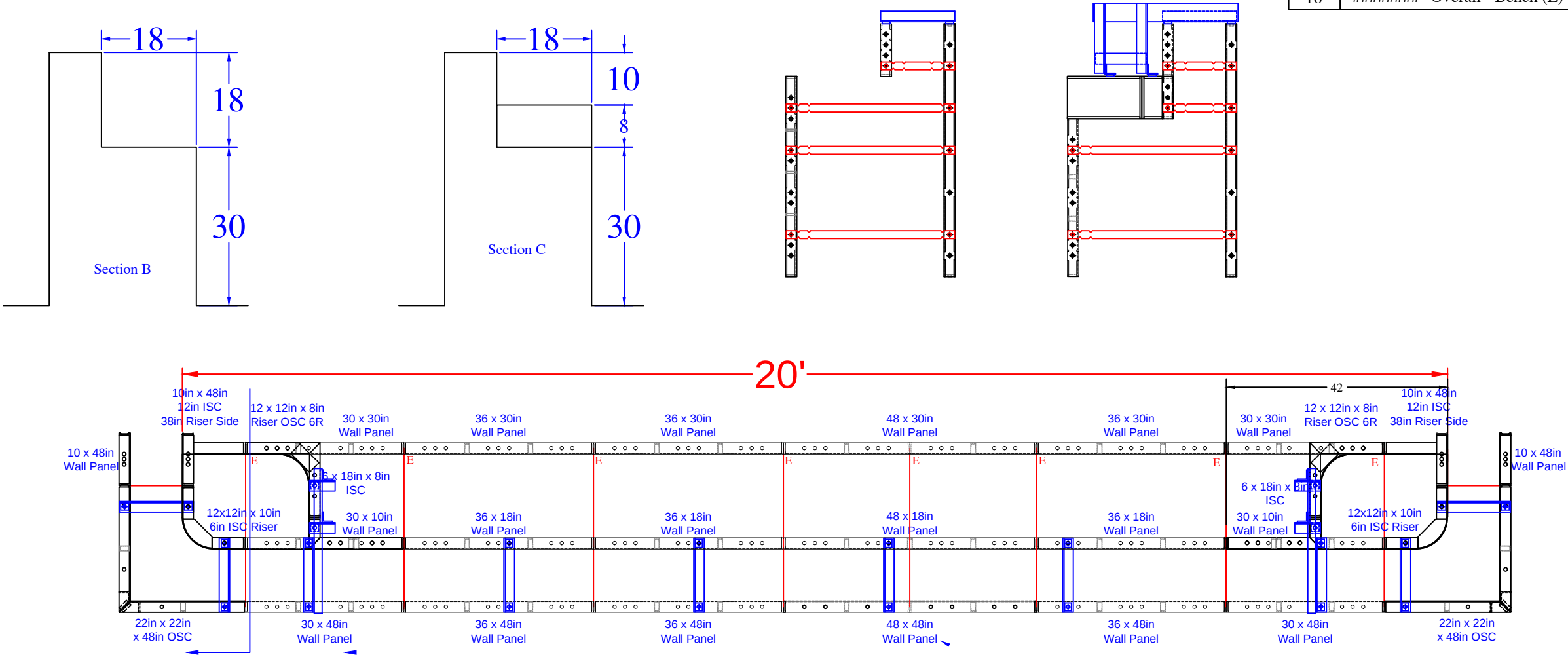
STEP & BENCH PANEL DETAIL
