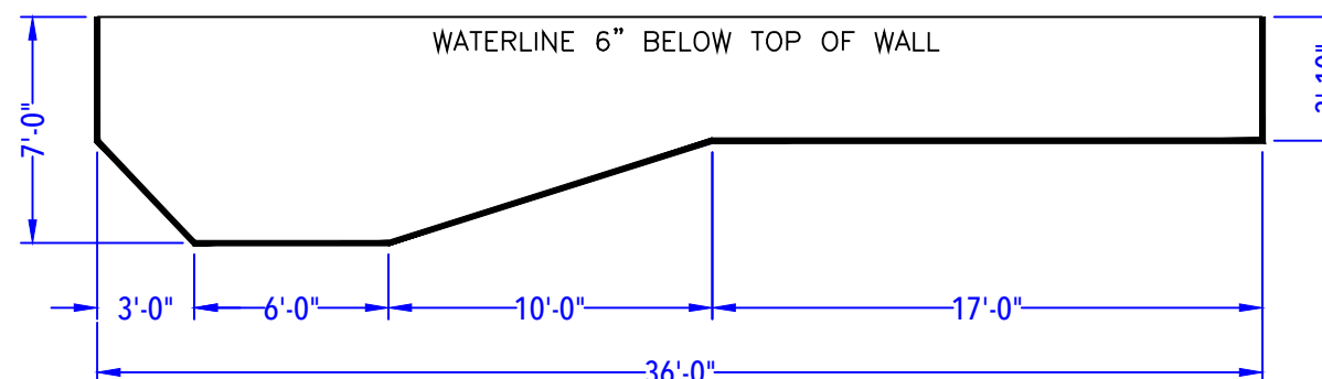
DEPTH DETAIL
