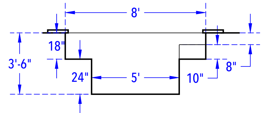
SPA ELEVATION (After Concrete & Plaster) N.T.S
