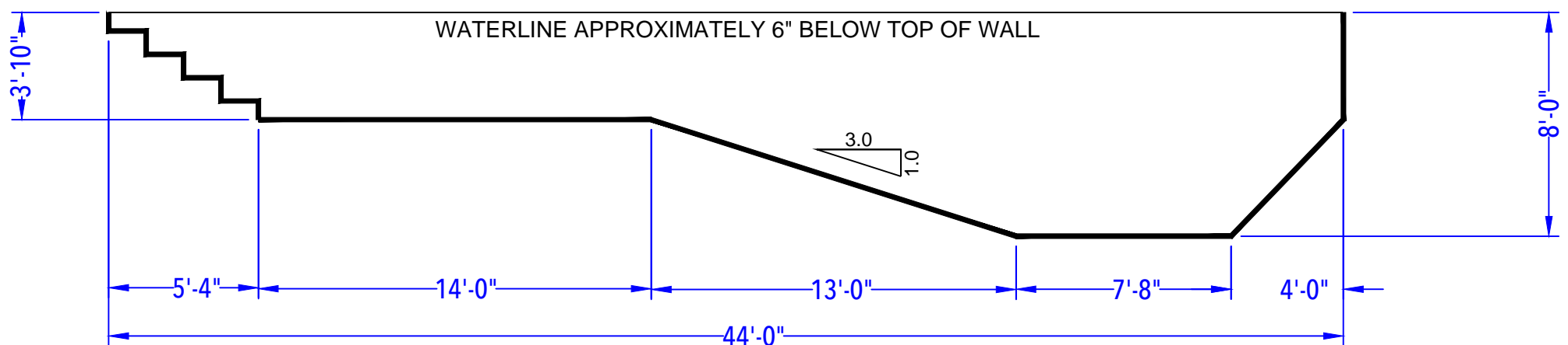
DEPTH DETAIL
