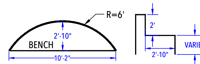
DEEP END BENCH & STEP OUT DETAIL (After Concrete & Liner) N.T.S.
