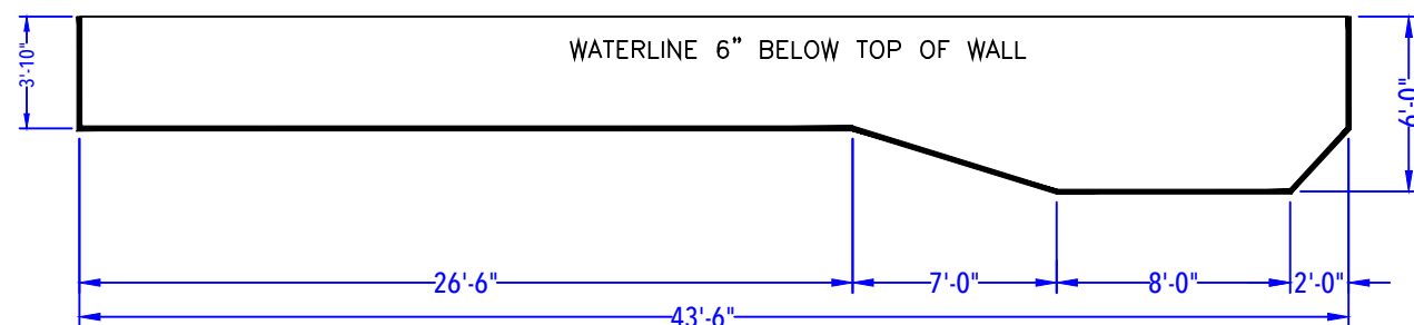
DEPTH DETAIL
