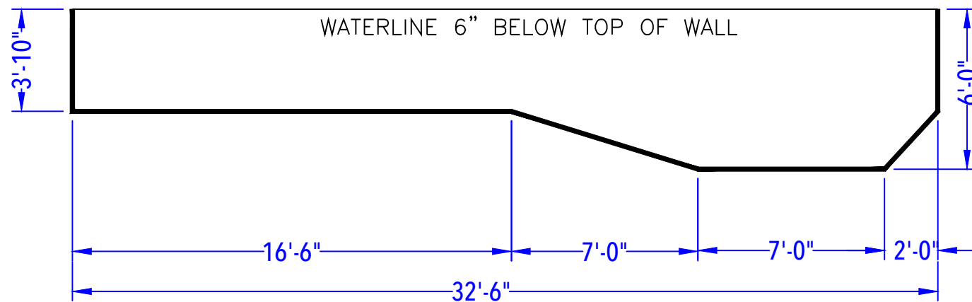
DEPTH DETAIL
