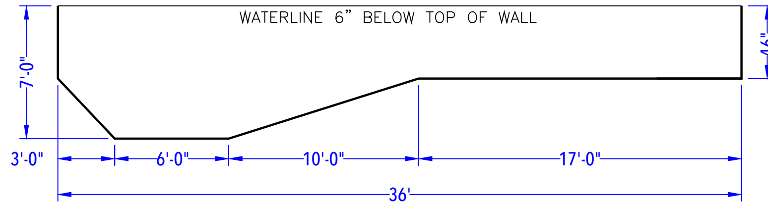
DEPTH DETAIL
