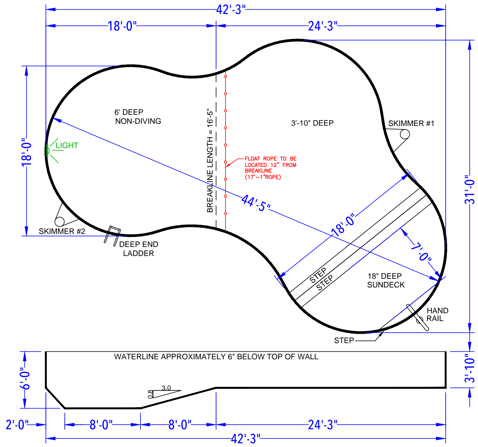
DEPTH DETAIL
