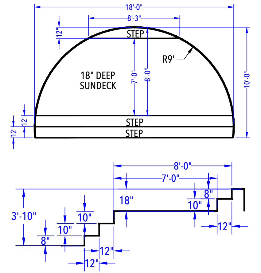
SUN DECK & ENTRY STEP DETAIL (After Concrete & Liner) N.T.S.
