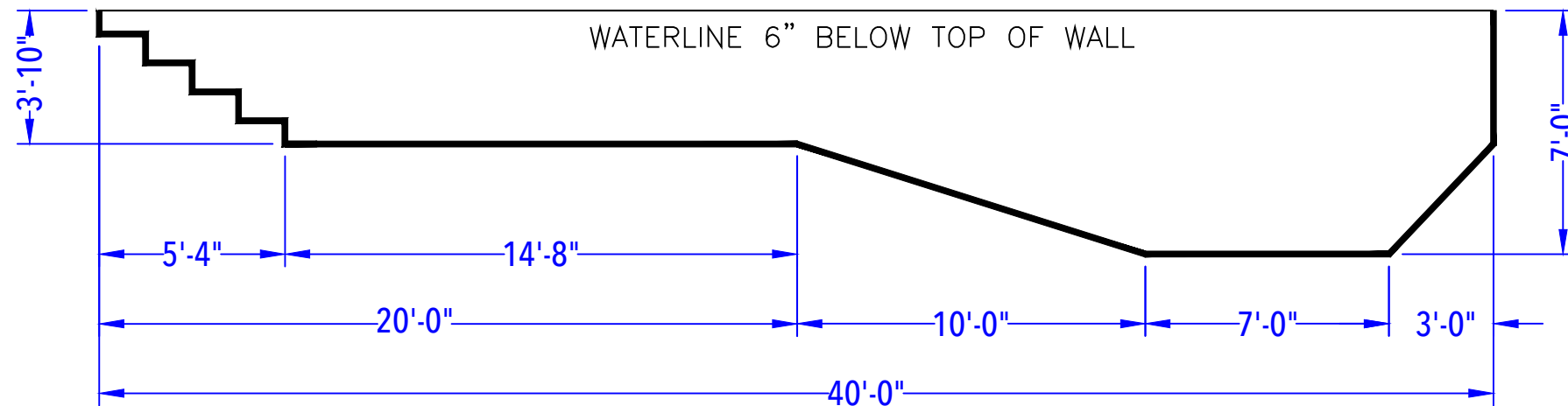
DEPTH DETAIL
