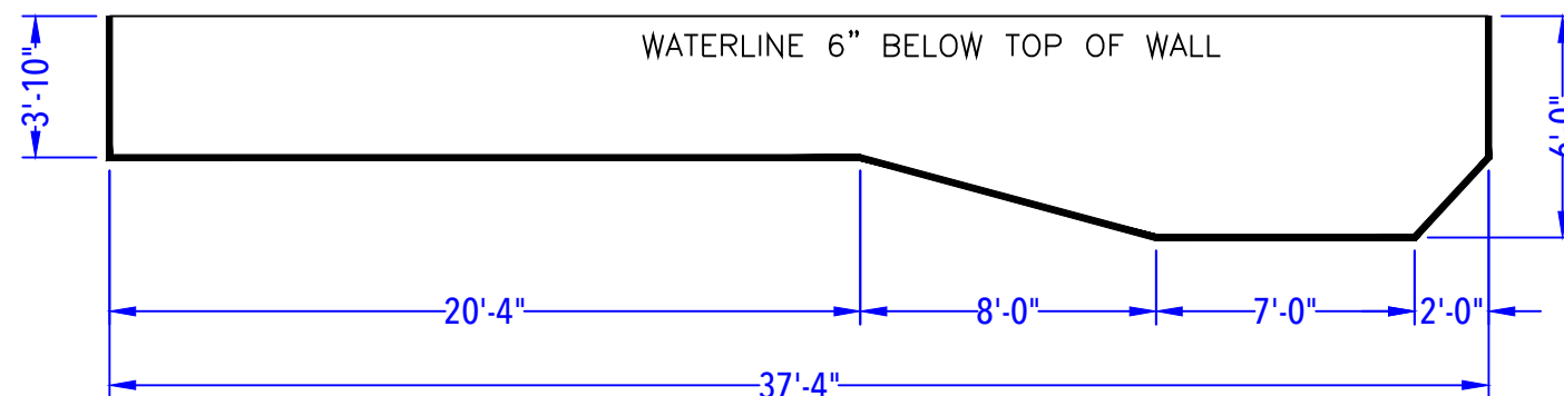
DEPTH DETAIL
