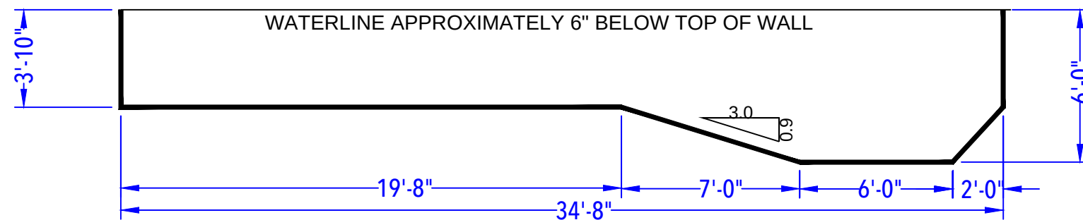
DEPTH DETAIL
