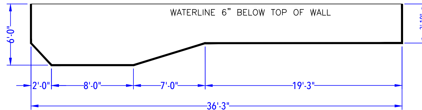
DEPTH DETAIL
